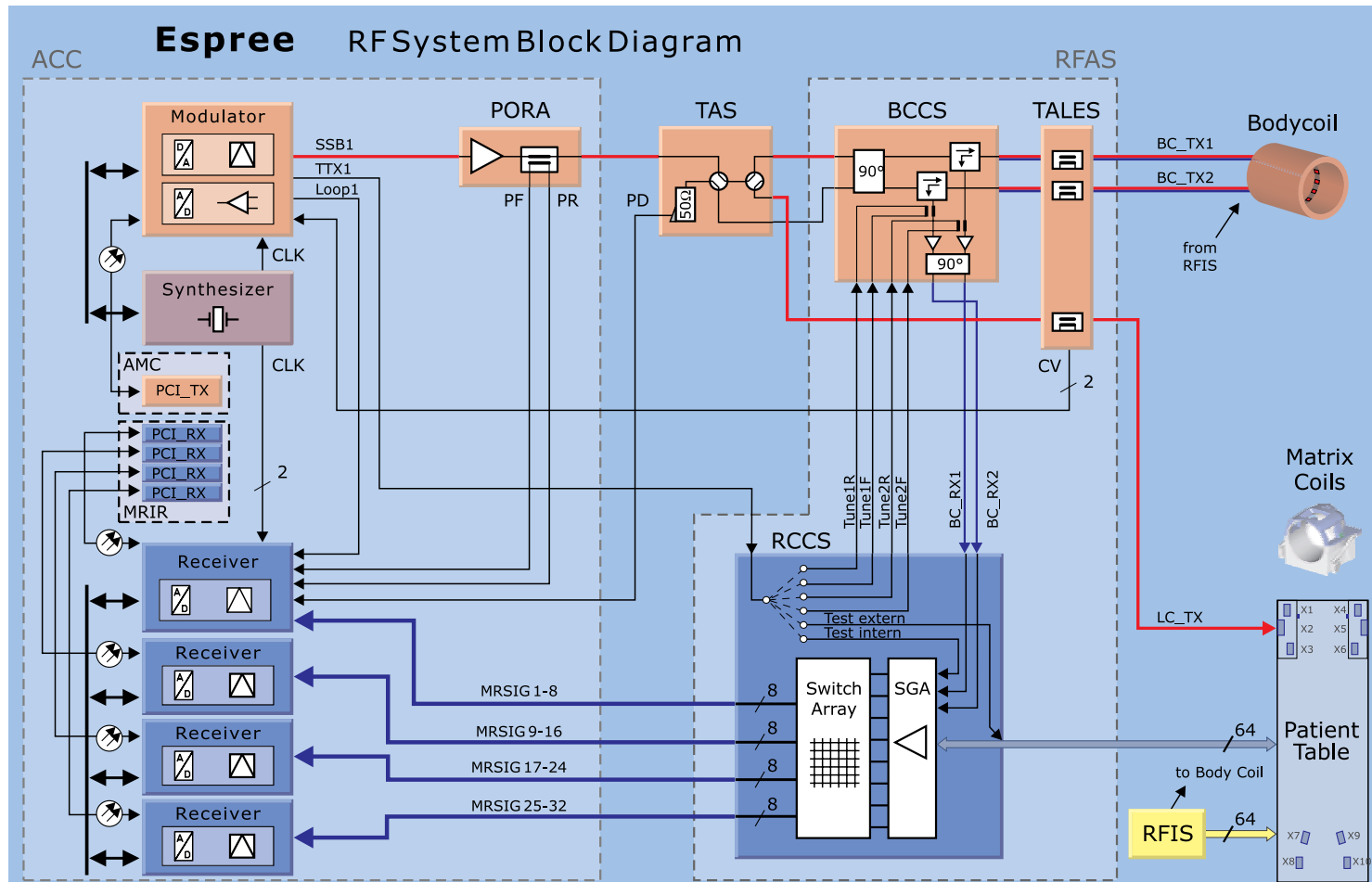
Fig. 115 Block Diagram of Espree RF System
